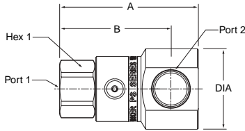
3 Piece Design
