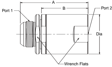
3 Piece Design
