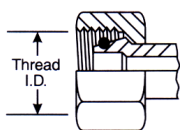
DIN Female "DKO" Style 12° Cone Seat (with O-Ring)
